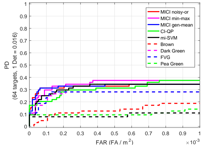
Fig. 4: The ROC curve for one run of train on campuses 1 and 4, test on campus 3.
